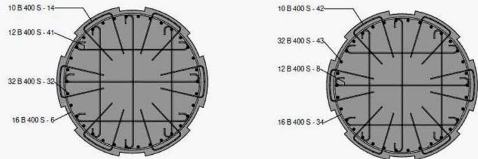
8 Pier 1 Reinforcement 1:25 9 Pier 2 Reinforcement 1:25
